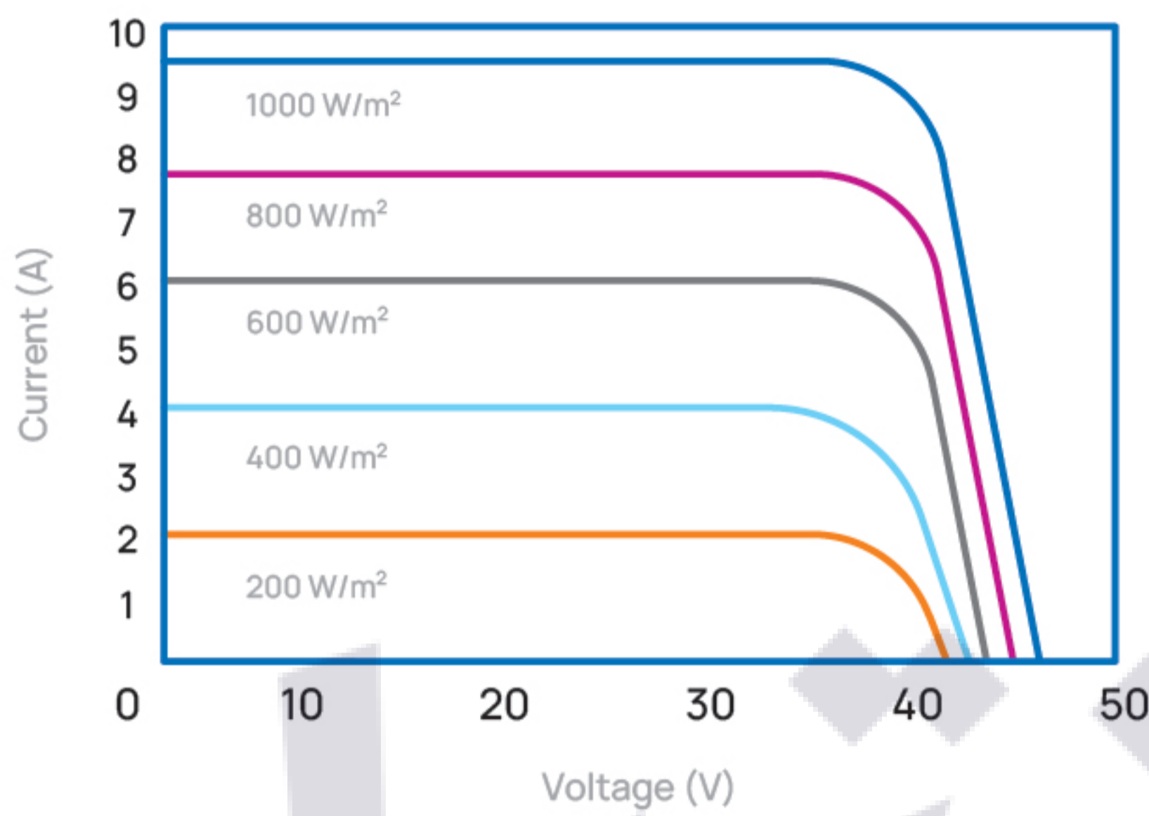
Current-Voltage Curve 390W
