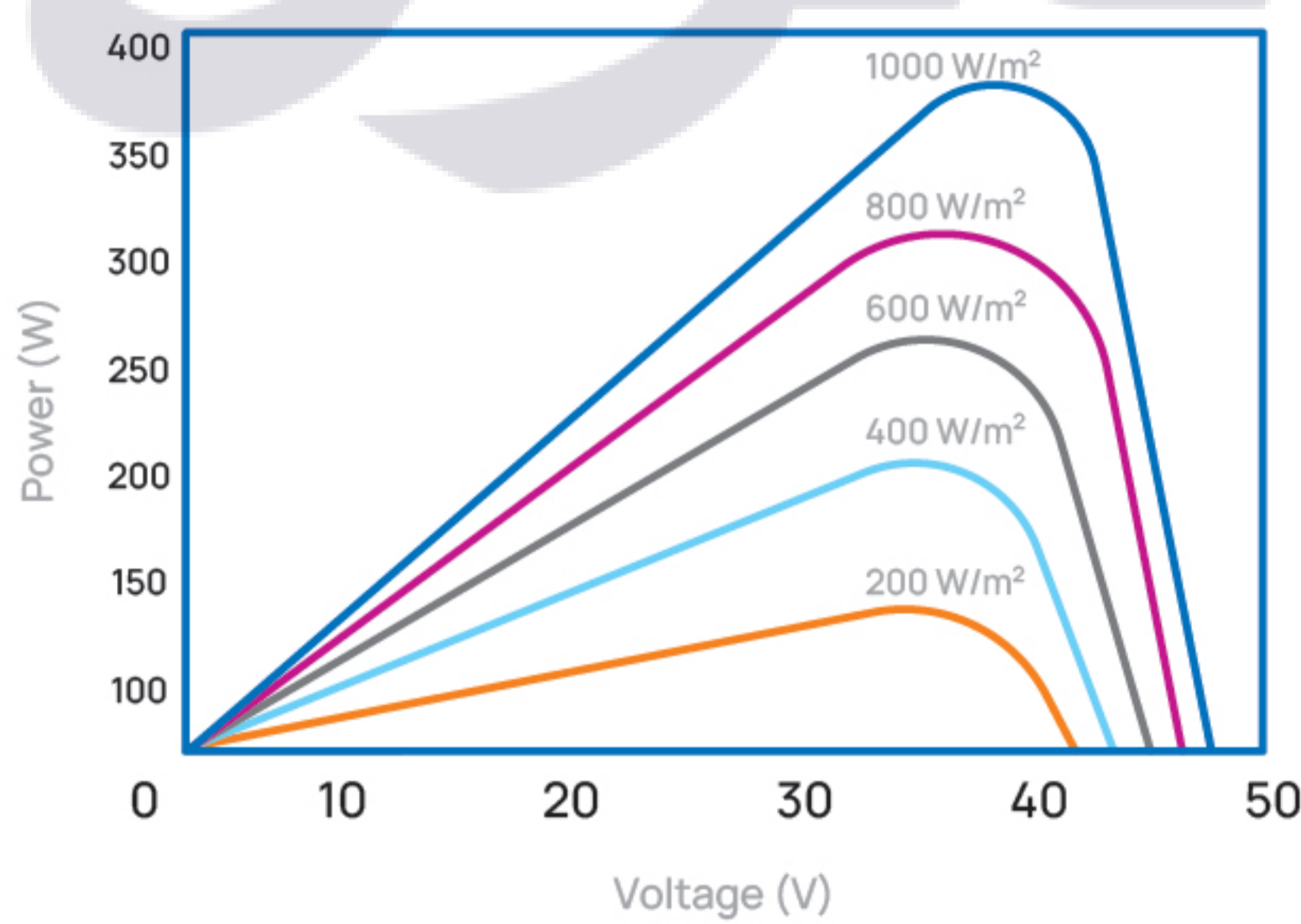
Power-Voltage Curve 390W
