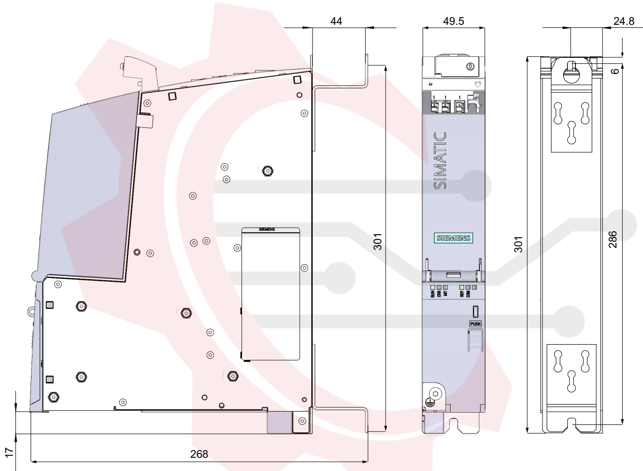
Figure A-1 Dimension drawing of SIMATIC Drive Controller
