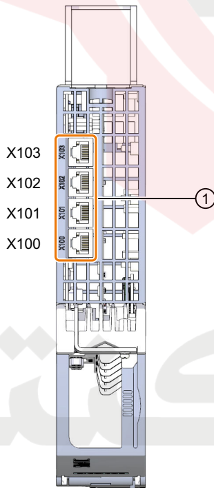
① X100 to X103: 4 x DRIVE-CLiQ interface
