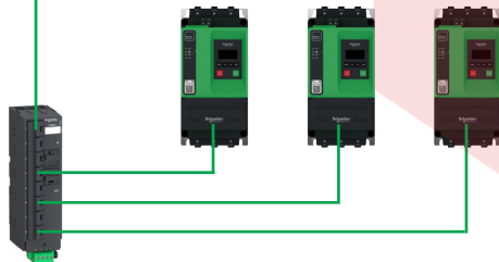
Firmware upload of several ATS430 soft starters at the same time through Modbus serial using Ecostruxure Automation Device Maintenance
